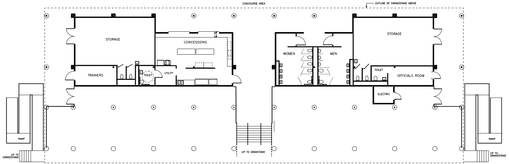
FLOOR PLAN OF CONCESSIONS BUILDING
